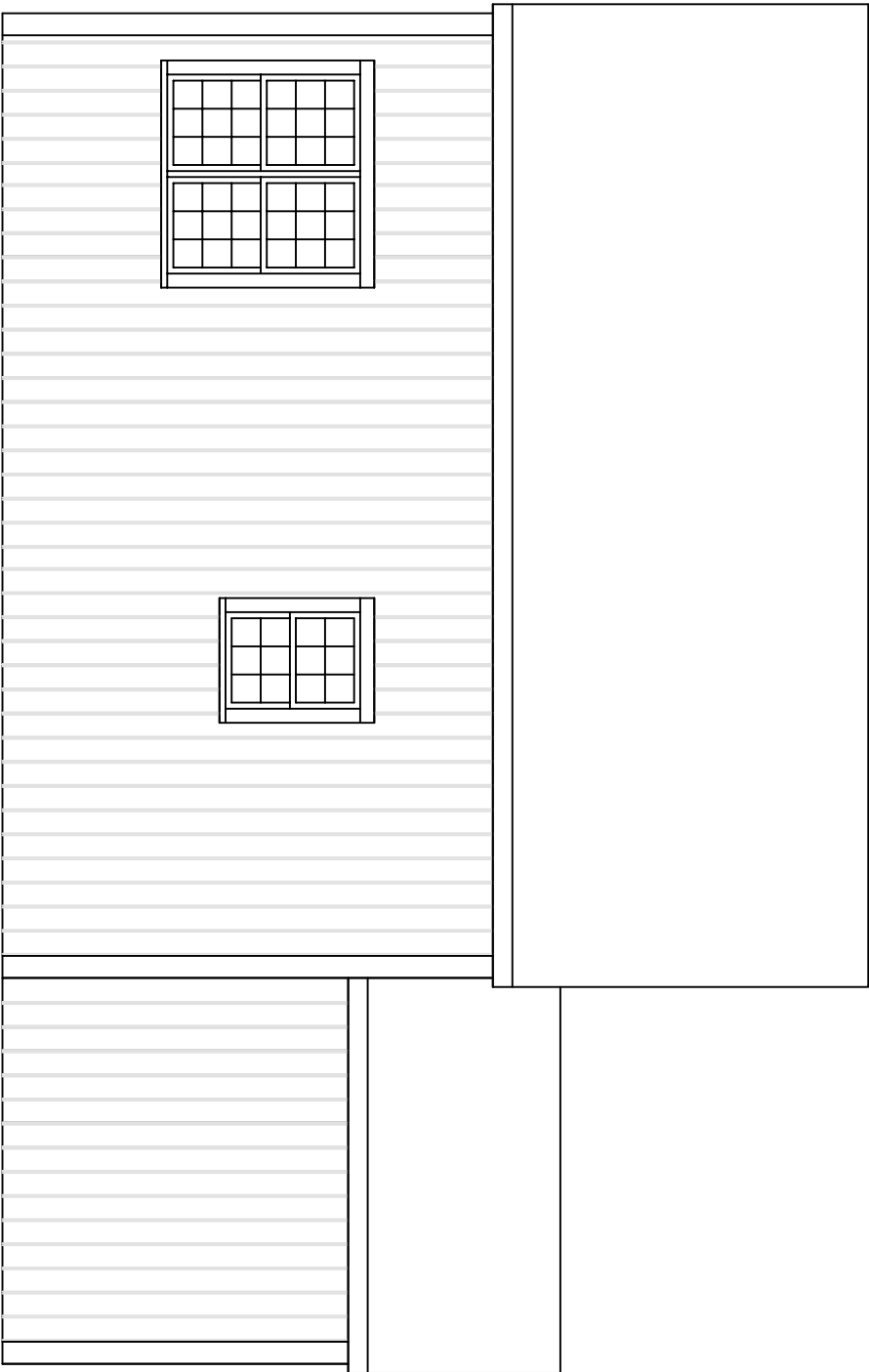
REAR ELEVATION
